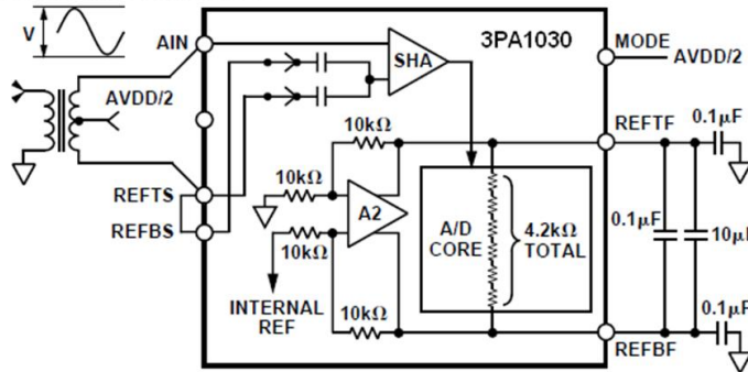
c. Differential Mode
