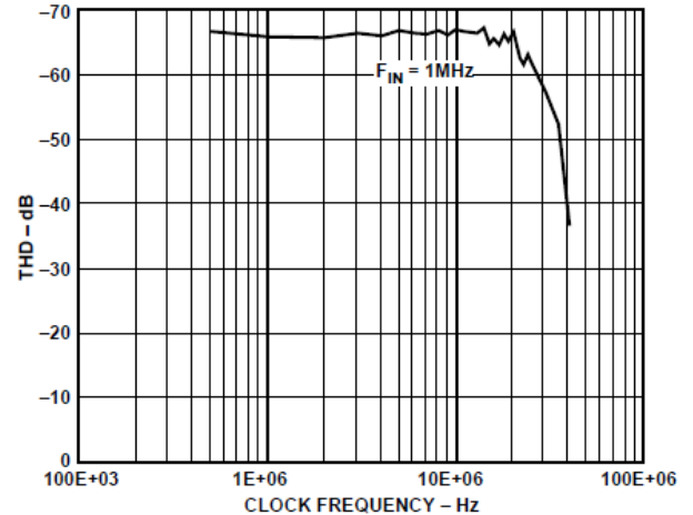
Figure 8. THD vs. Clock Frequency
