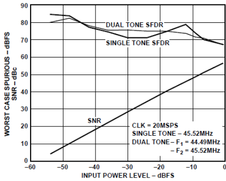
Figure 28. SNR/SFDR for IF @ 45 MHz
