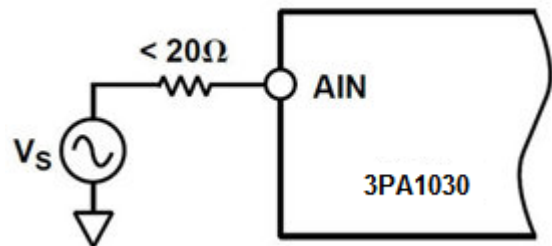
Figure 20. Simple 3PA1030 Drive Configuration
