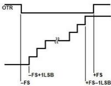
Figure 25. Output data format
