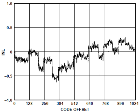
Figure 4. Typical INL
