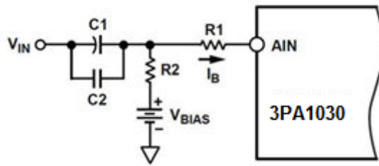
Figure 21. AC Coupled Input
