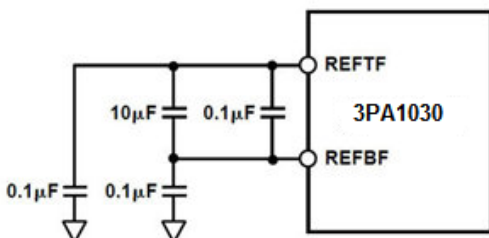
Figure 13. Reference Decoupling Network
