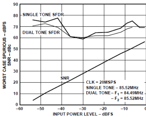
Figure 30. SNR/SFDR for IF @ 85 MHz
