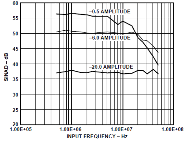
Figure 6. SINAD vs. Input Frequency
