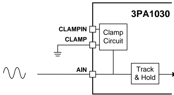
Figure 18-c, DC-coupled input
