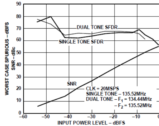
Figure 31. SNR/SFDR for IF @ 135 MHz
