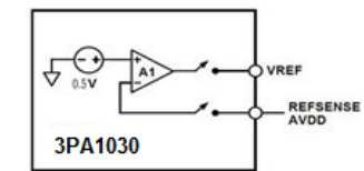
g. Internal Reference Disable (Power Reduction)
