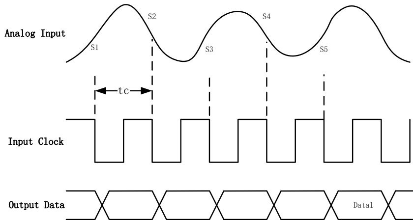
Figure 24. Timing Diagram
