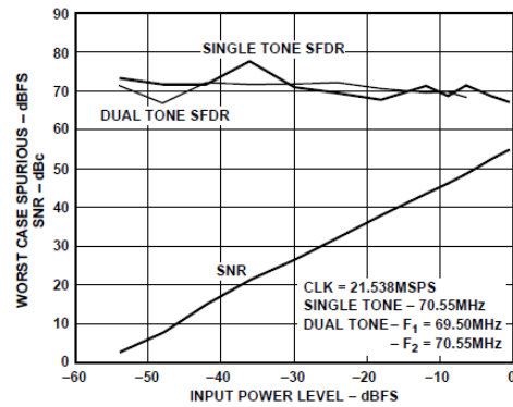
Figure 29. SNR/SFDR for IF @ 70 MHz
