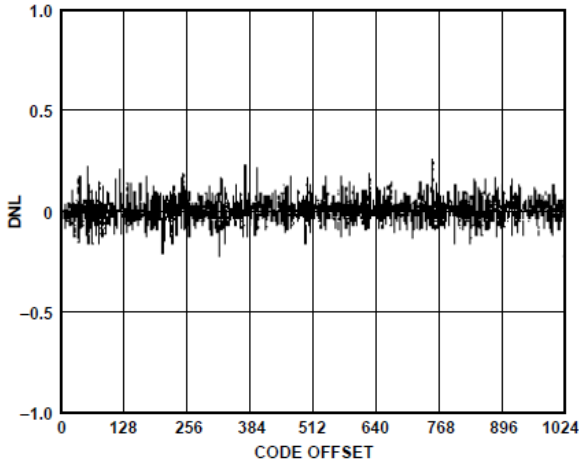
Figure 3. Typical DNL
