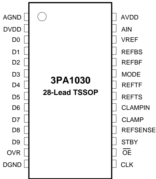
Figure 2. Pin Location
