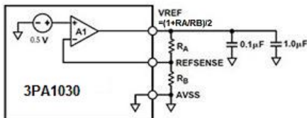
f. Variable Reference (Between 0.5 V and 1 V)
